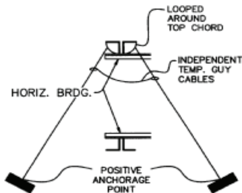
HORIZONTAL BRIDGING TERMINUS POINT SECURED BY TEMP. GUY CABLES
