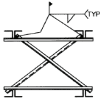
JOISTS PAIR BRIDGING TERMINUS POINT
