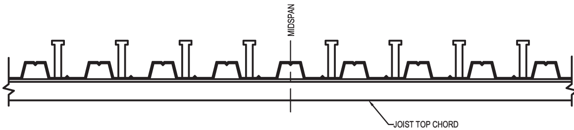
SHEAR STUD LAYOUT IN "STRONG" POSITION
