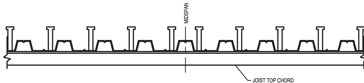
SHEAR STUD LAYOUT IN "WEAK" POSITION
