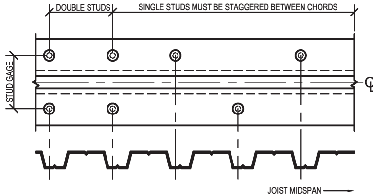
SINGLE AND DOUBLE SHEAR STUD POSITION ON TOP CHORD
